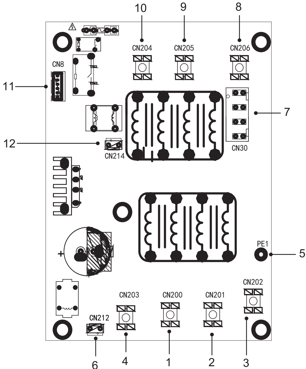
PCB C
